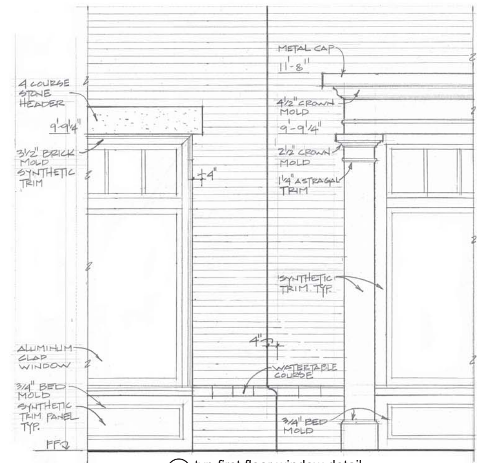
1 typ first floor window detail 1/4" = 1'-0"
